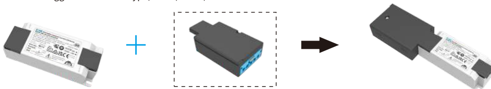
Model: BK-BAS010A Pluggable connector type: WAGO(770-2115/007-000)
