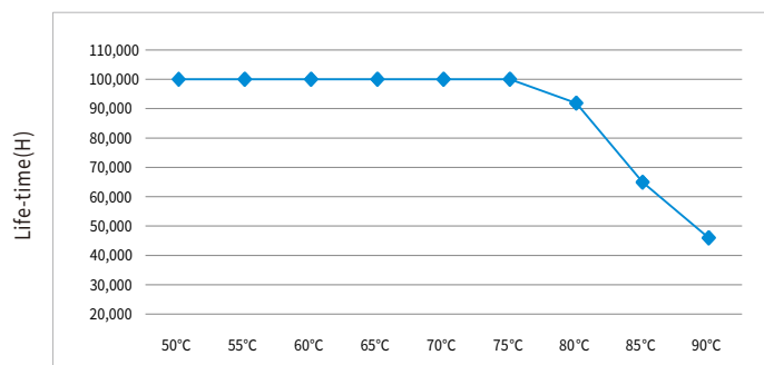
BK-KUL050-1300Am
