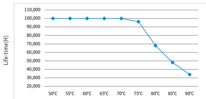
BK-KUL060-1650Am
