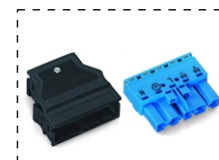
Pluggable connector other side: WAGO(770-1105/022-000)
